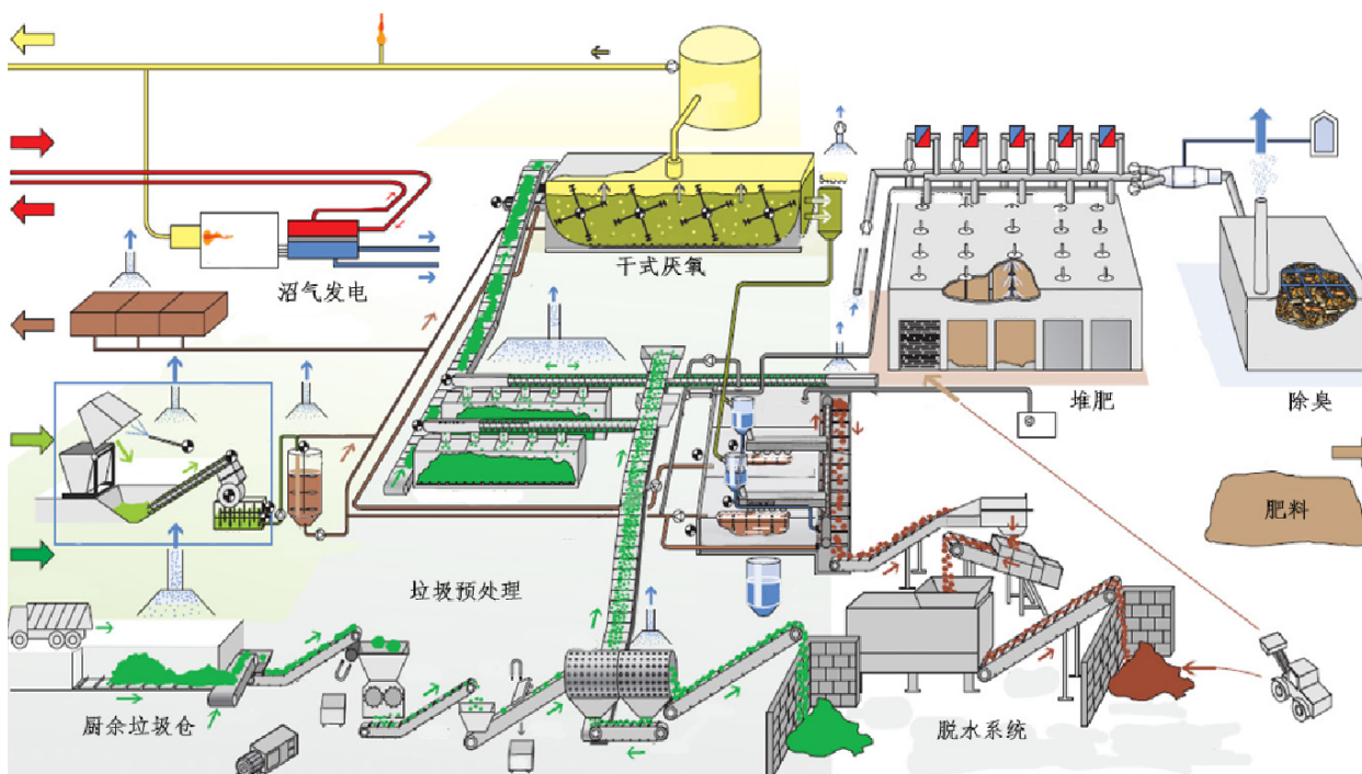
Figure 3-10 Process Roadmap of Fuzhou Food Waste Treatment Plant
